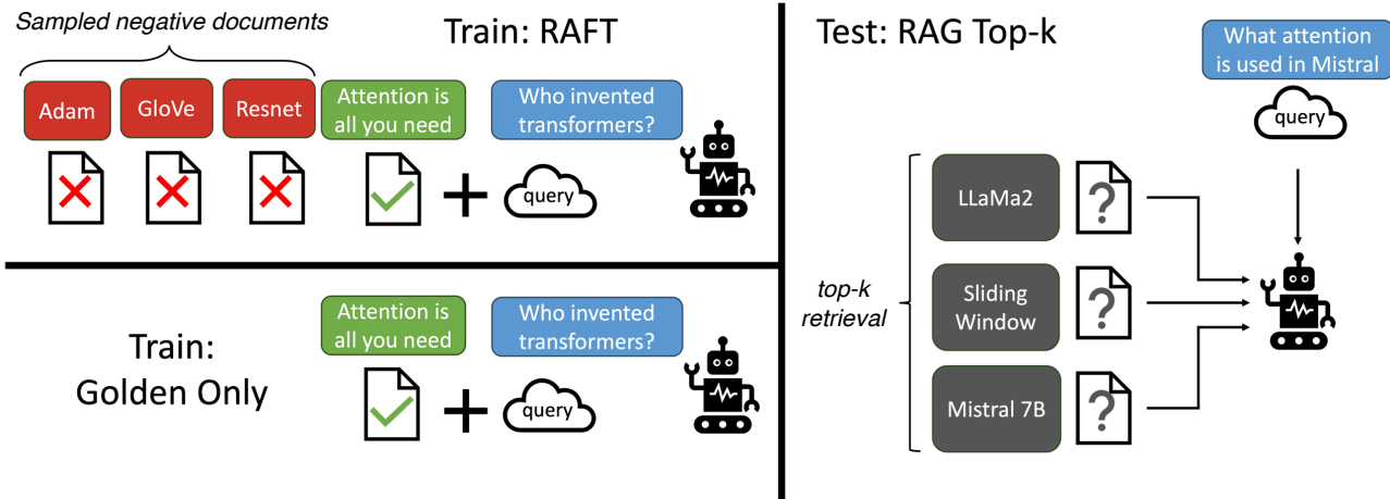
Figure 11: RAFT training method (Image taken from [17])
